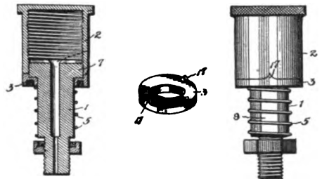
BOWEN GREASE CUP CAP LOCK.
